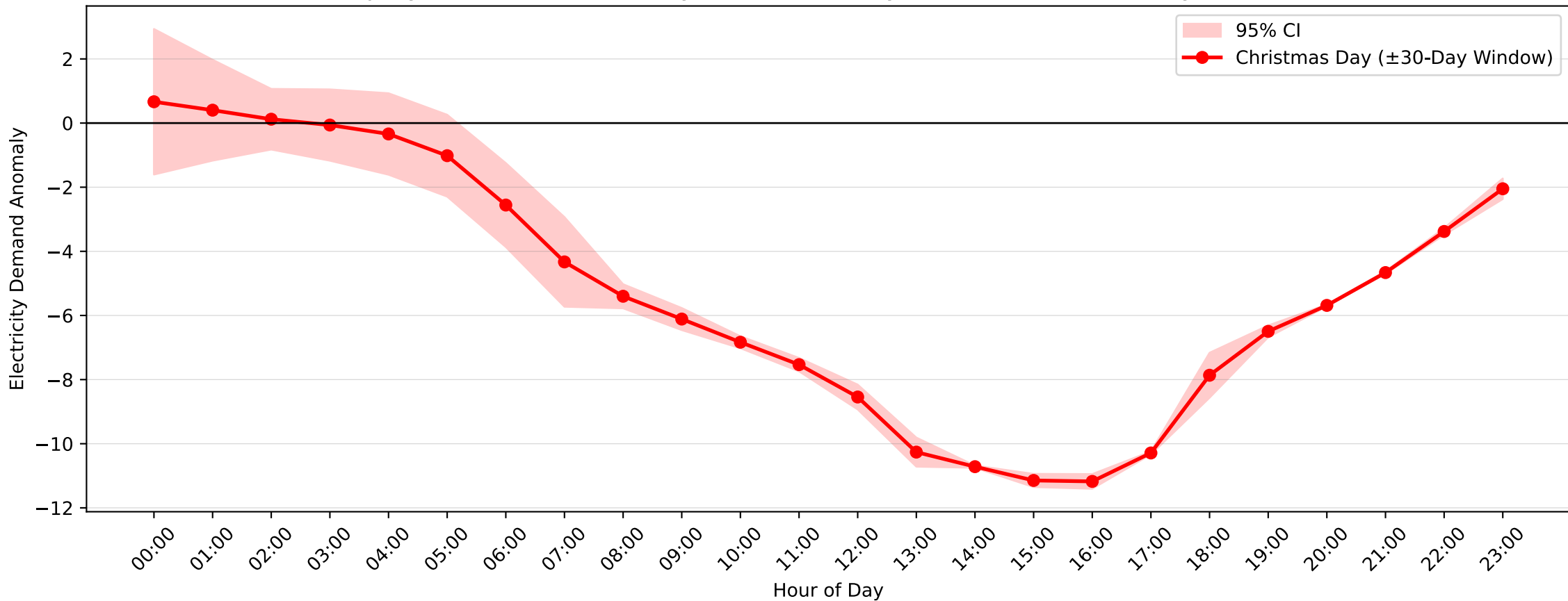
Top Ryde Demand Anomaly: Christmas Day (2012-2013, \pm 30 -Day Window)
