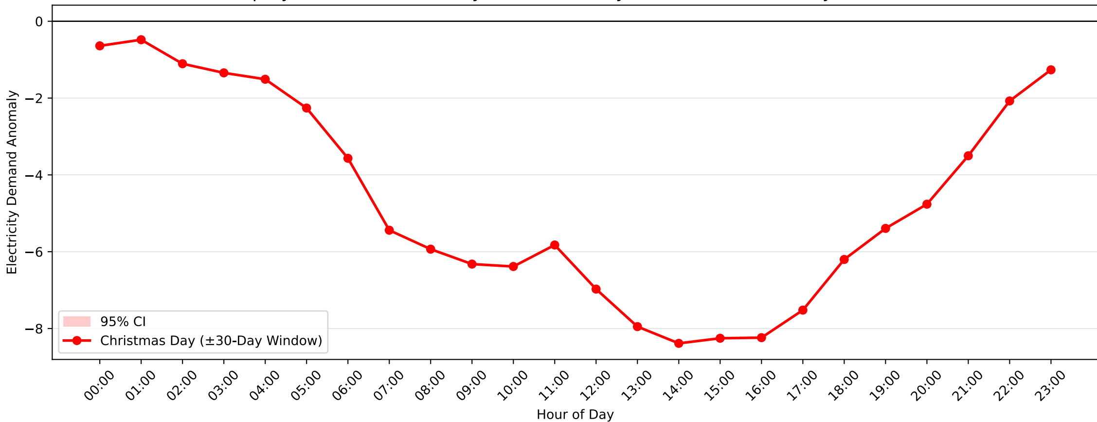
Top Ryde Demand Anomaly: Christmas Day (2016-2017, \pm 30 -Day Window)
